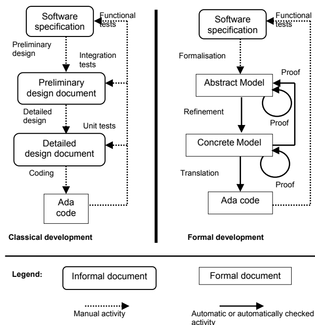
Figure 1: Comparison of the classical and formal development cycle
