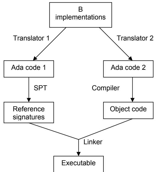
Figure 2: Translating B to Ada
